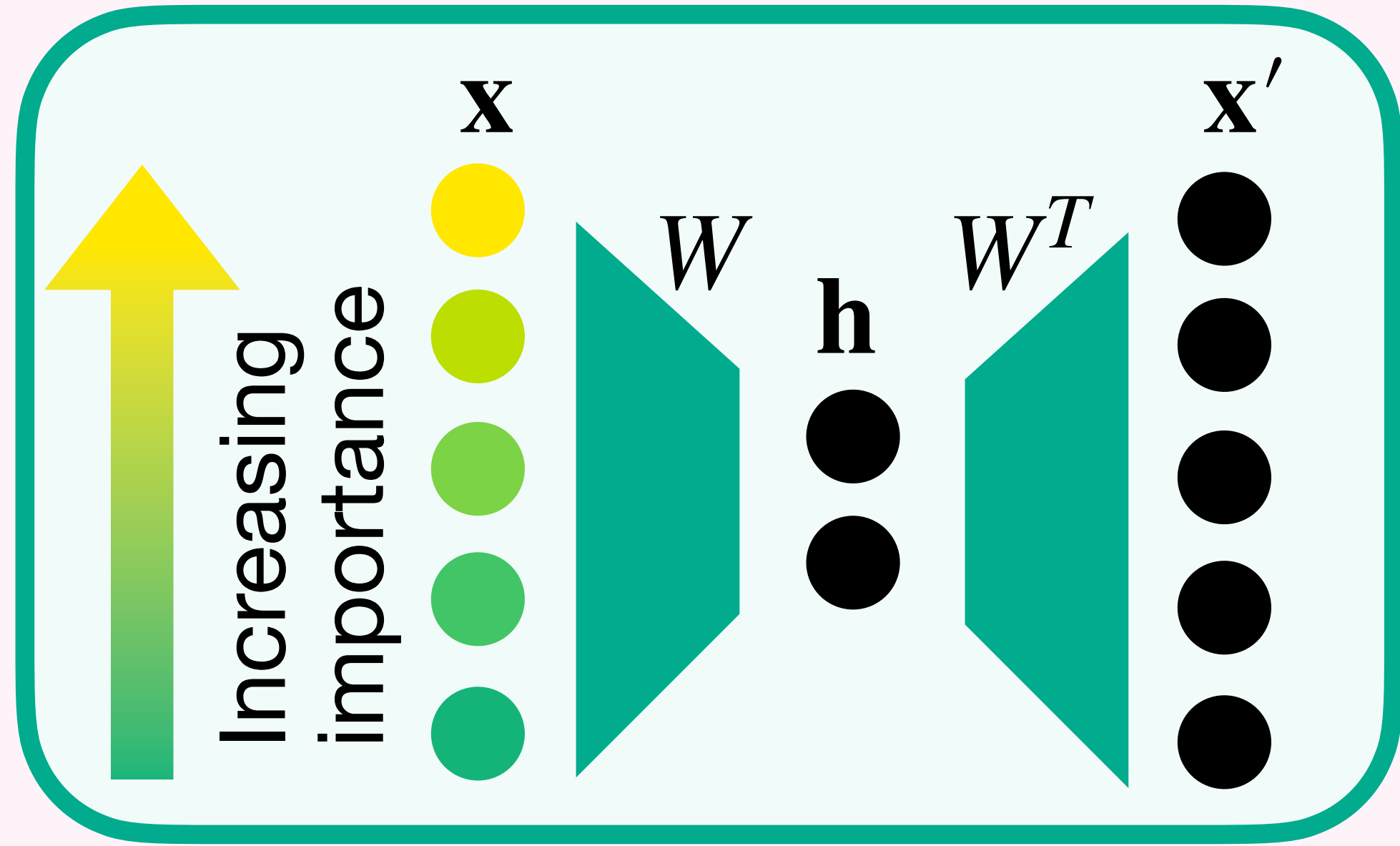
Toy model architecture
