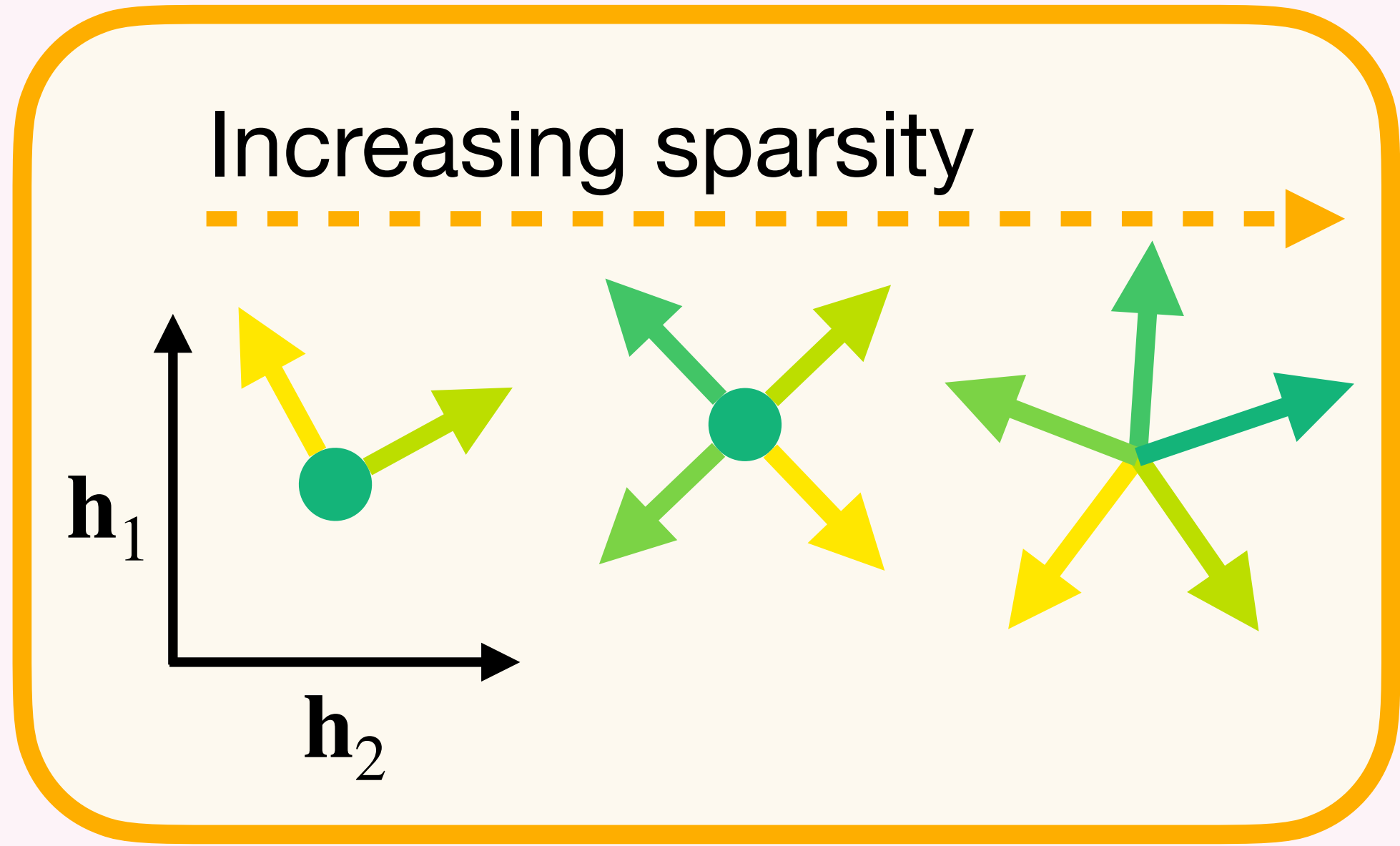
Effect of sparsity
